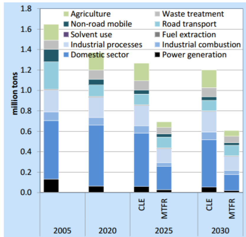
Figure 3.3: PM2.5 emissions of the TSAP 2013 Baseline; Current legislation (CLE) and Maximum Technically Feasible Reductions (MTFR), EU-28
